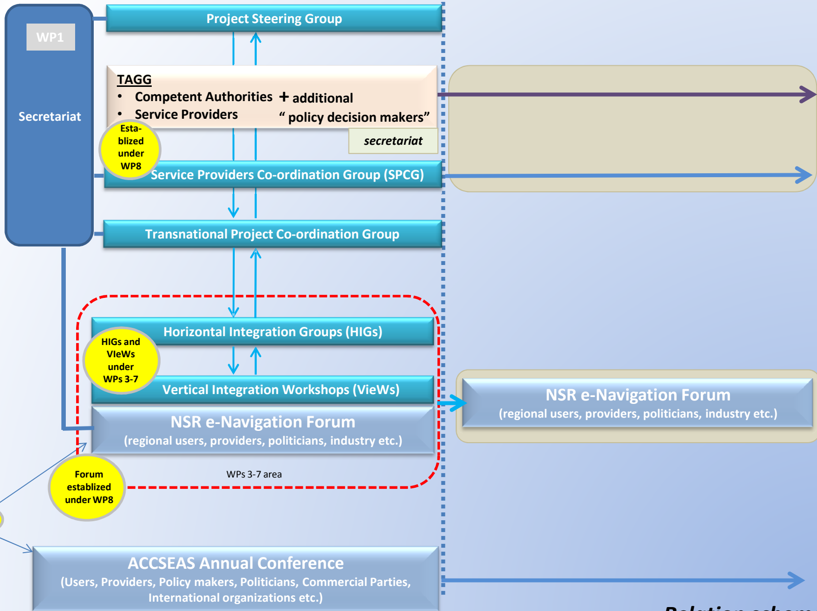
Relation scheme
